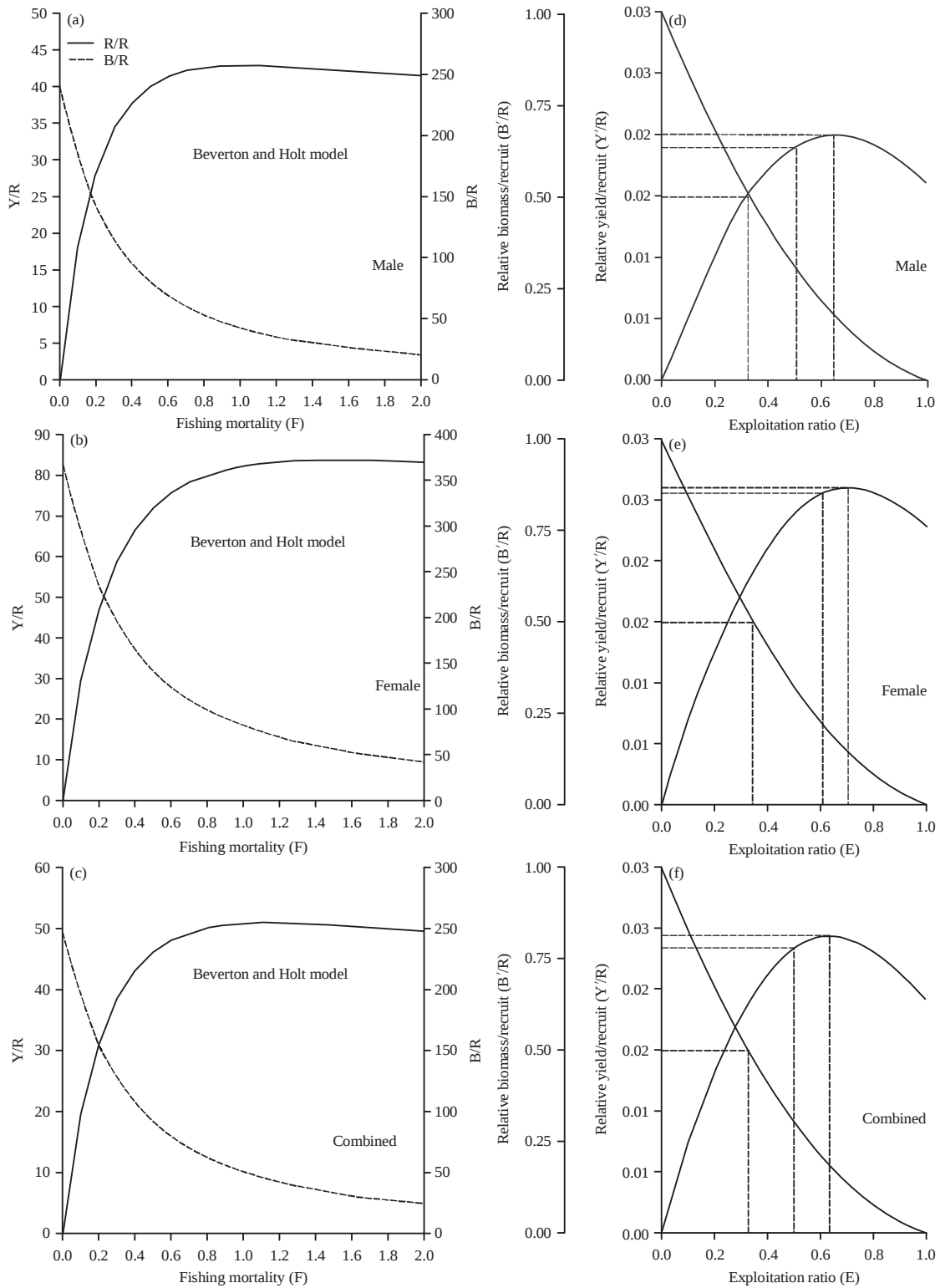
Fig. 7(a-f): (a-c) Yield per recruit (Y/R) and biomass per recruit (B/R) and (d-f) Relative yield per recruit (Y'/R) and biomass per recruit (B'/R) of Oreochromis niloticus in El-Bahr El-Faraouny Canal
